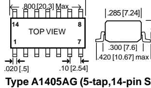
Type A1405AG (5-tap, 14-pin SM)
