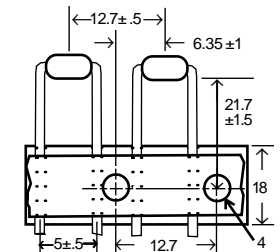
Horiz. Preform (Code THP) 1/8 & mini-1/4W body sizes
