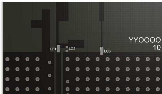
3D View of matching components and recommended values (LC1=00hm, LC2=OPEN, LC3=8.2nH)
